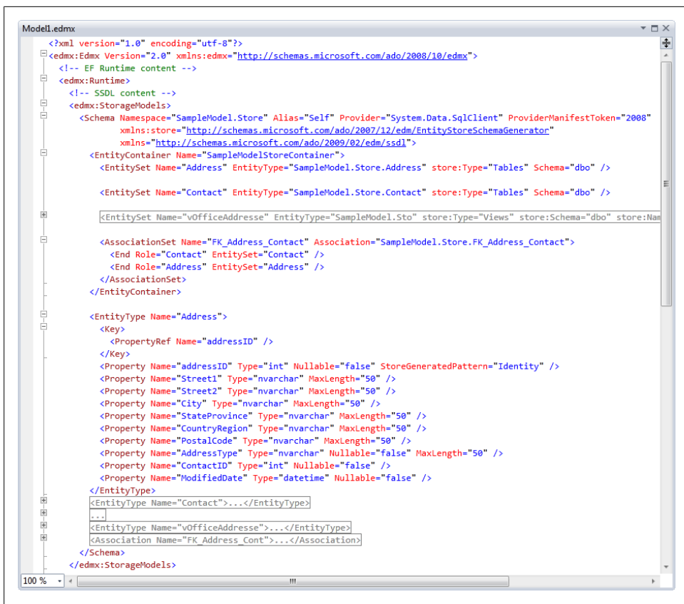
Figure 2-17. Expanded StorageModels section to explore the store layer of the model
