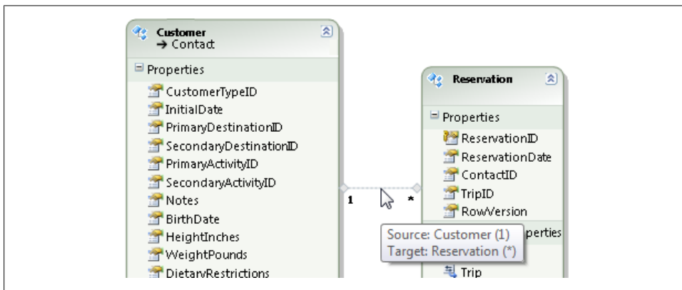
Figure 19-1. An association represented in the Designer
