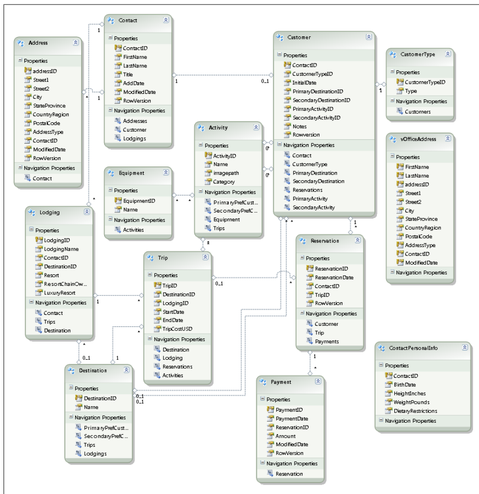
Figure 8-8. The BreakAway model that you will use in chapters that follow
