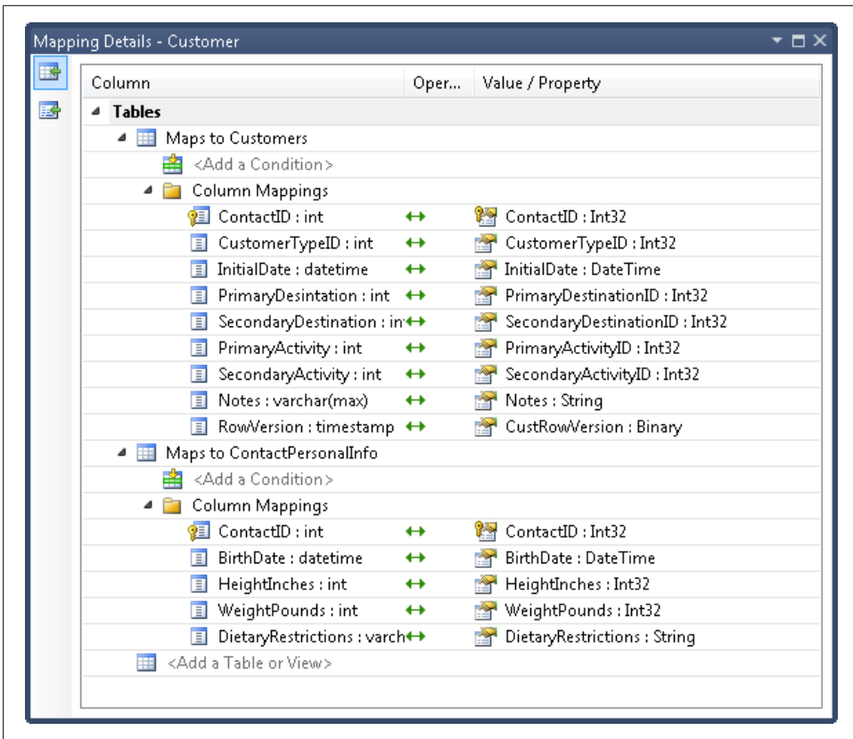
Figure 14-9. Mapping an entity to multiple tables
