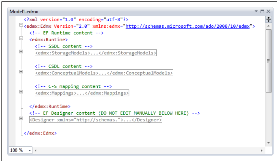
Figure 2-9. The main sections of the model
